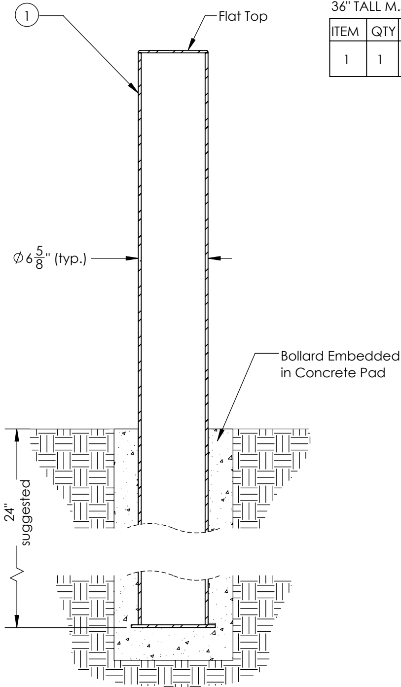
36" TALL M.S. BOLLARD SLEEVE
