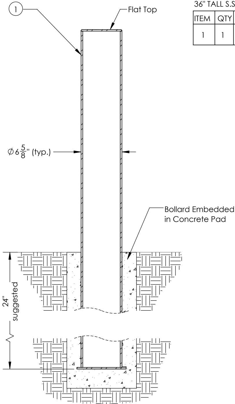
36" TALL S.S. BOLLARD SLEEVE
