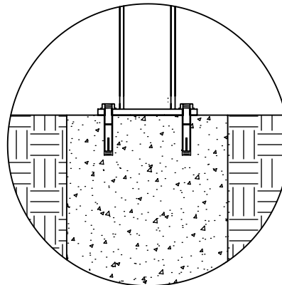
TYPE B Bolt Down Mount
