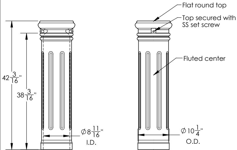
TYPE D Deep Mount
