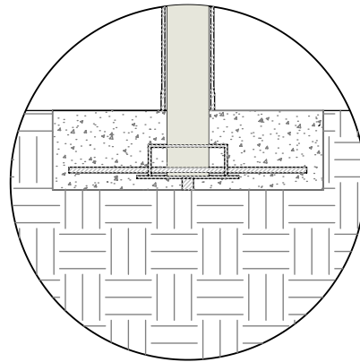
TYPE S Shallow Mount
