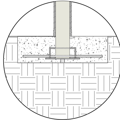
TYPE CR1 Shallow Mount
