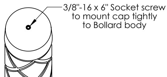
Top View of Bollard Cap
