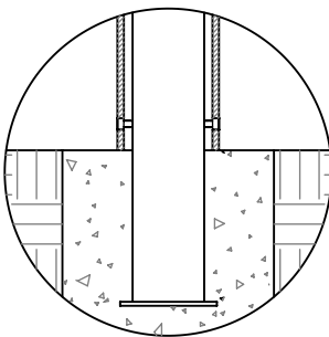
TYPE P Pipe Mount
