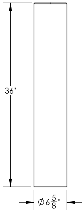
TYPE P Pipe Mount
