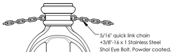
Optional Eye Bolt and Chain
