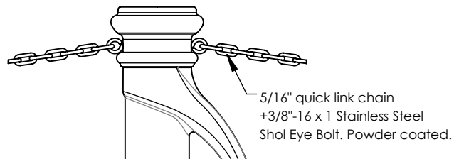
Optional Eye Bolt and Chain
