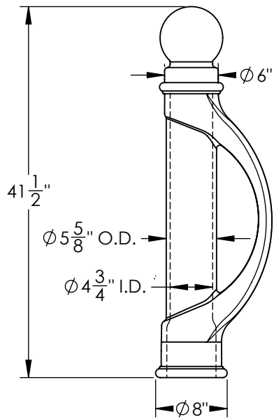
TYPE P Pipe Mount
