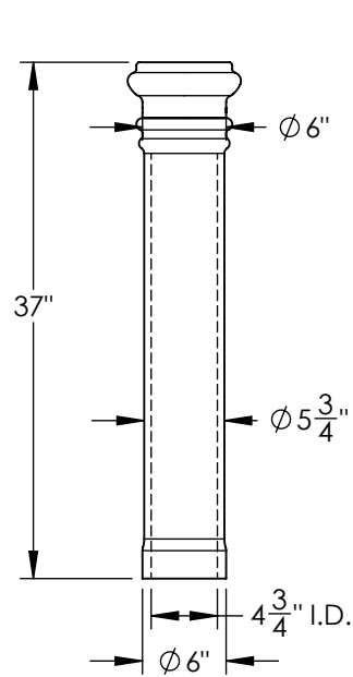
TYPE P Pipe Mount
